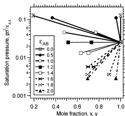
Figure 9. Vapor–liquid coexistence diagram for several mixtures differing in \epsilon_{AB} , as indicated. The lines join a single pair of coexistence points (each for a system of an overall mole fraction (vapor + liquid + interface) of 0.7) to a common coexistence point for the pure-solvent system. All data are for T = 1.0 .
